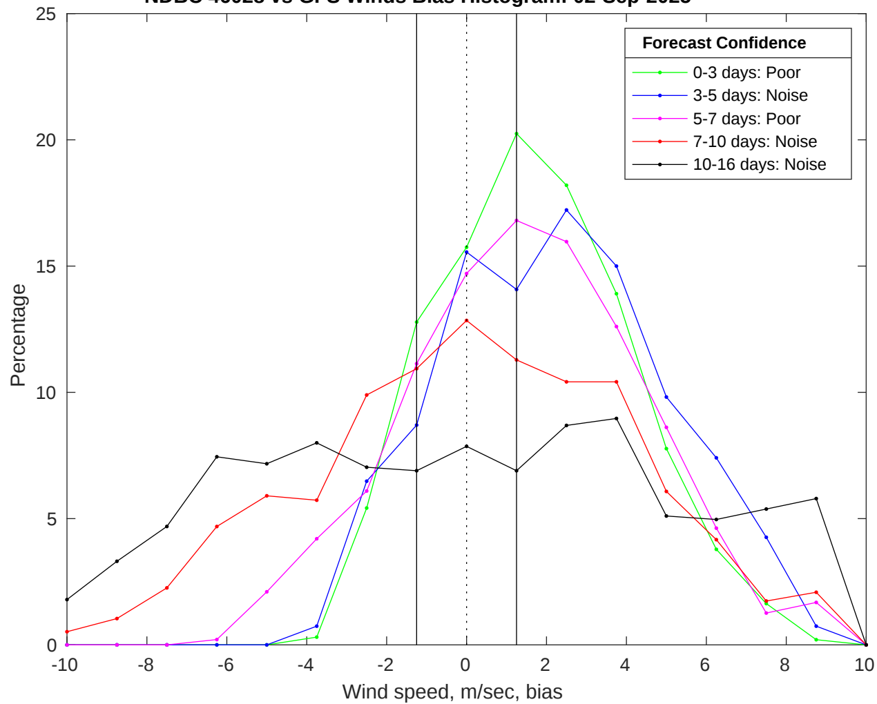
NDBC 46028 vs GFS Winds Bias Histogram: 02-Sep-2025
