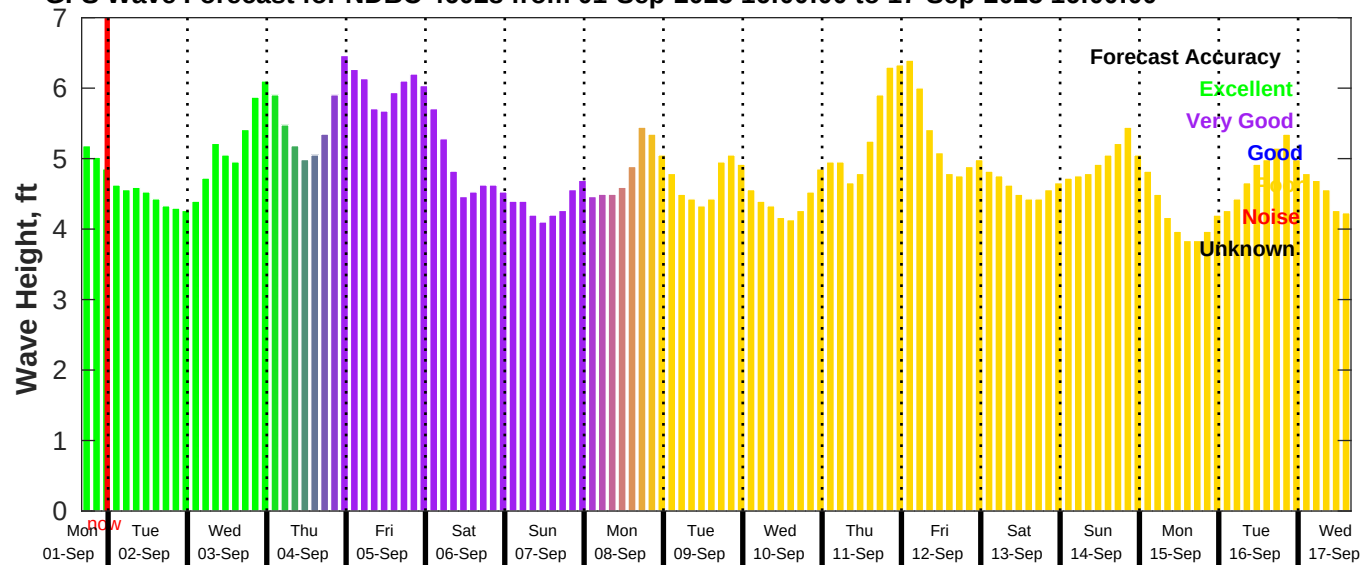
GFS Wave Forecast for NDBC 46028 from 01-Sep-2025 16:00:00 to 17-Sep-2025 16:00:00
