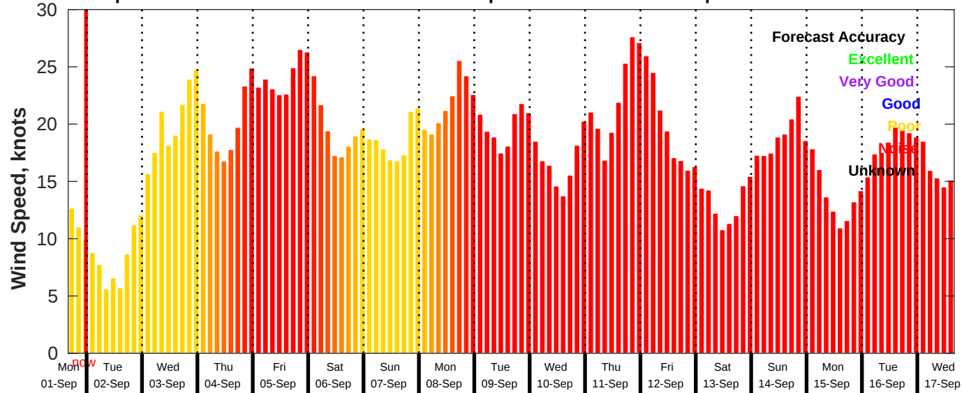
GFS Wind Speed Forecast for NDBC 46028 from 01-Sep-2025 16:00:00 to 17-Sep-2025 16:00:00
