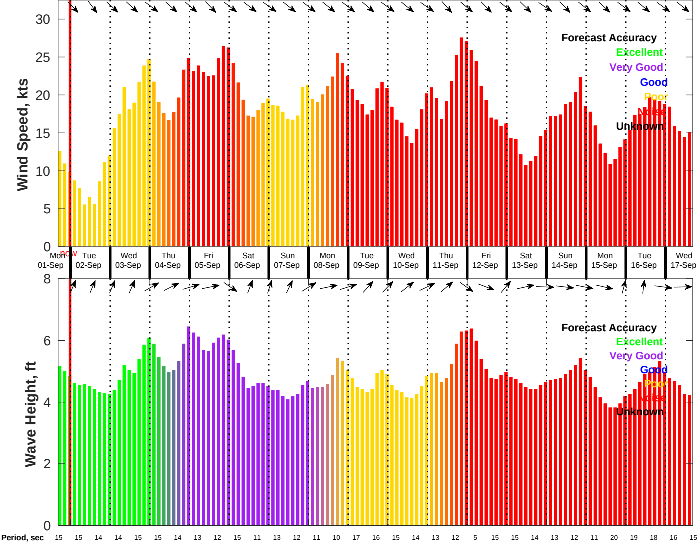
Wind & Wave Forecast for NDBC 46028 from 01-Sep-2025 16:00:00 to 17-Sep-2025 16:00:00
