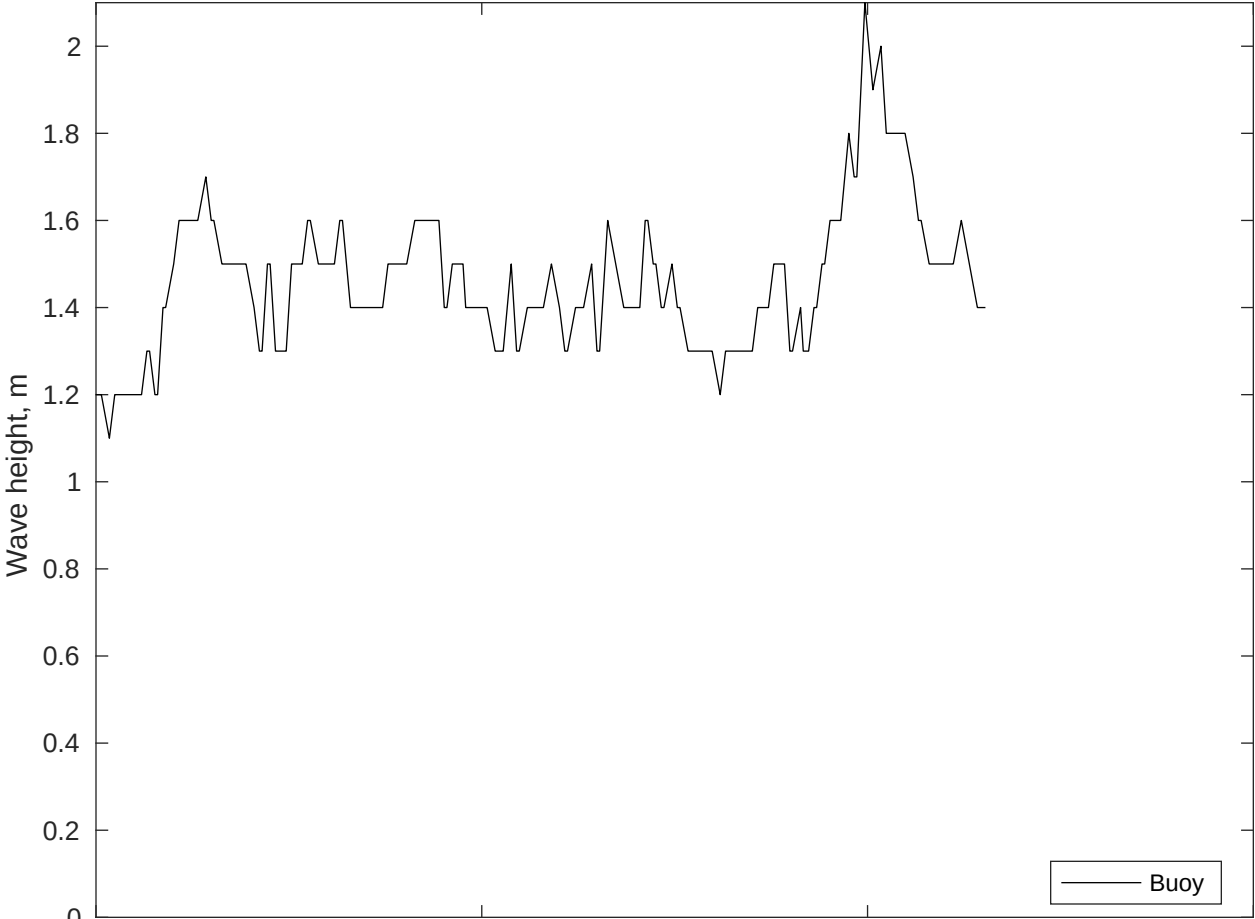
NDBC 46054 vs CMEMS Waves: 10 to 16 day forecast
