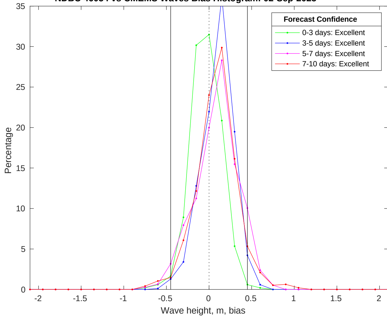
NDBC 46054 vs CMEMS Waves Bias Histogram: 02-Sep-2025
