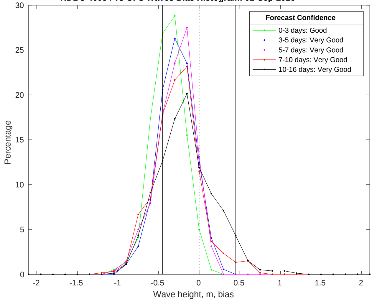
NDBC 46054 vs GFS Waves Bias Histogram: 02-Sep-2025
