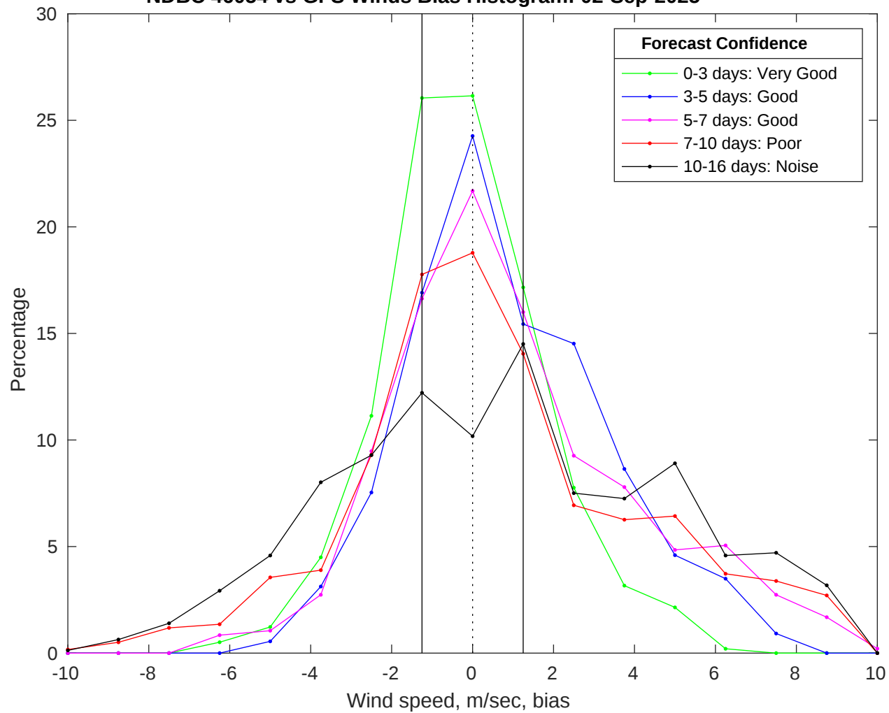
NDBC 46054 vs GFS Winds Bias Histogram: 02-Sep-2025
