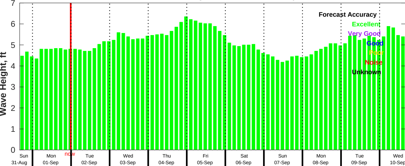
CMEMS Wave Forecast for NDBC 46054 from 31-Aug-2025 16:00:00 to 10-Sep-2025 16:00:00
