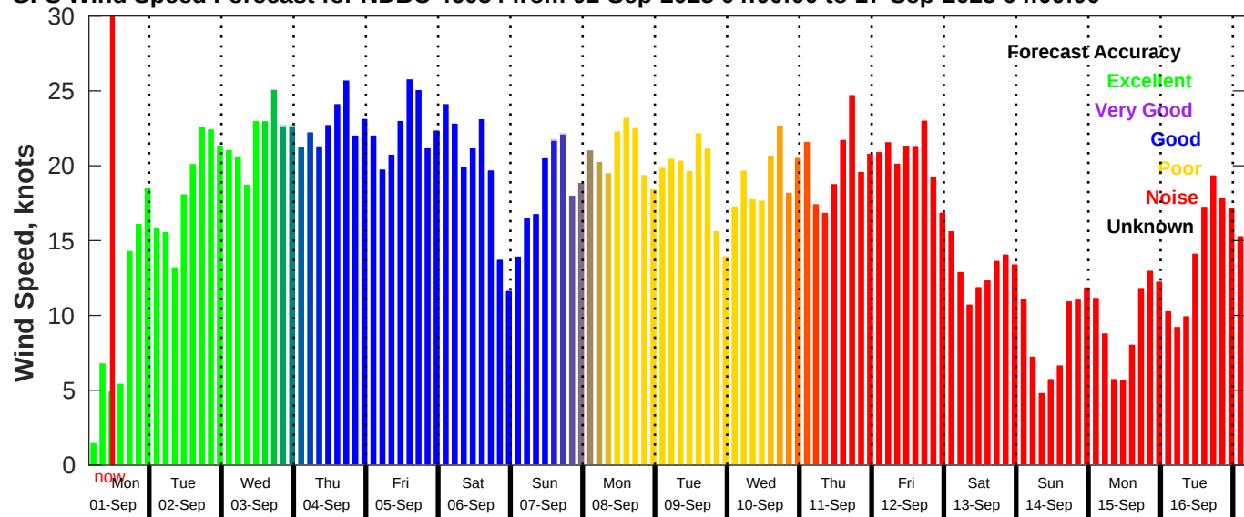
GFS Wind Speed Forecast for NDBC 46054 from 01-Sep-2025 04:00:00 to 17-Sep-2025 04:00:00
