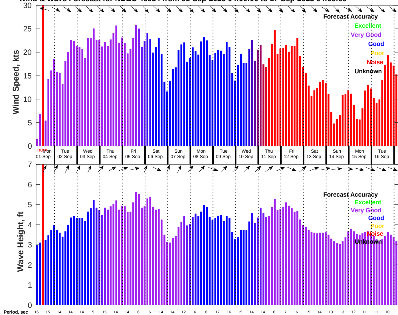
Wind & Wave Forecast for NDBC 46054 from 01-Sep-2025 04:00:00 to 17-Sep-2025 04:00:00
