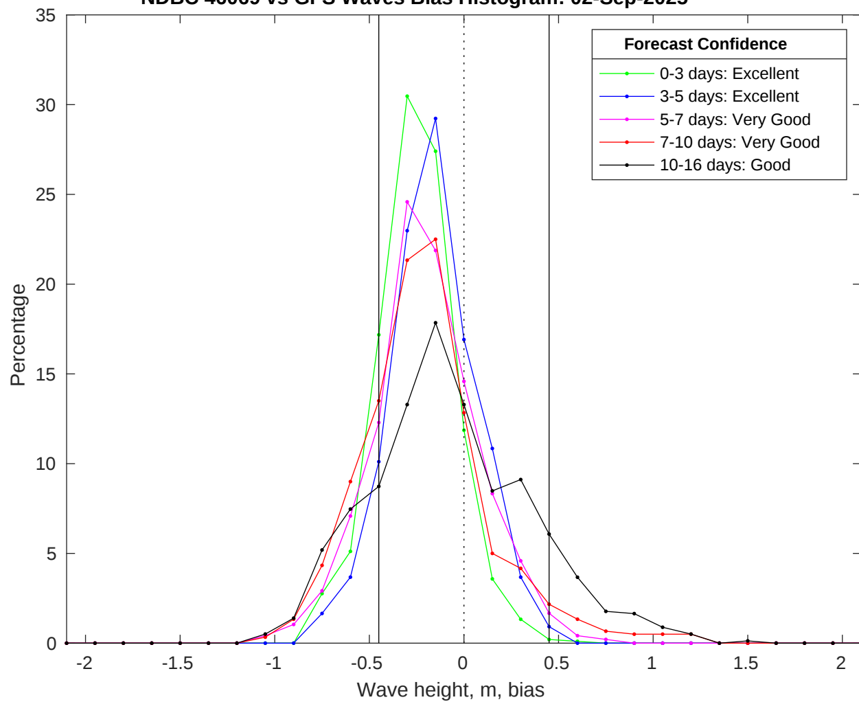
NDBC 46069 vs GFS Waves Bias Histogram: 02-Sep-2025
