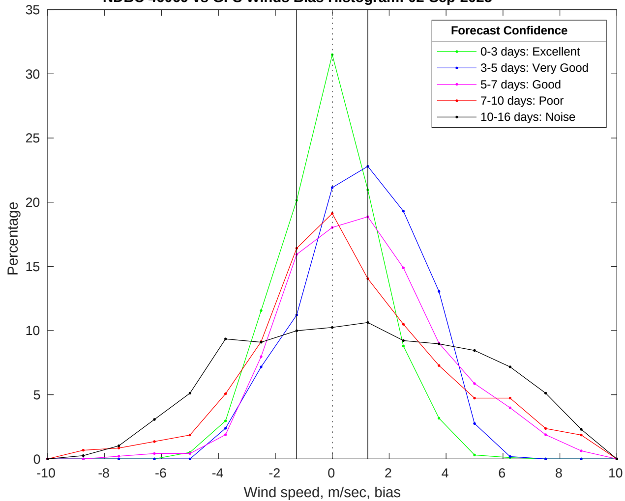
NDBC 46069 vs GFS Winds Bias Histogram: 02-Sep-2025
