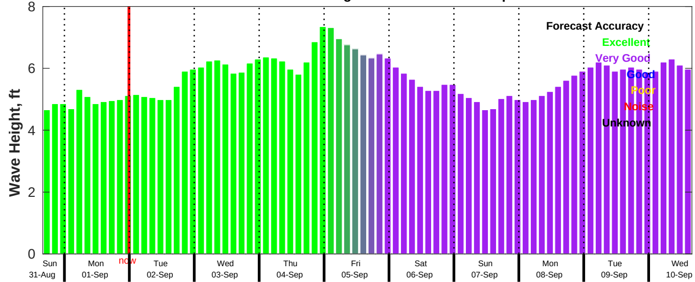
CMEMS Wave Forecast for NDBC 46069 from 31-Aug-2025 16:00:00 to 10-Sep-2025 16:00:00
