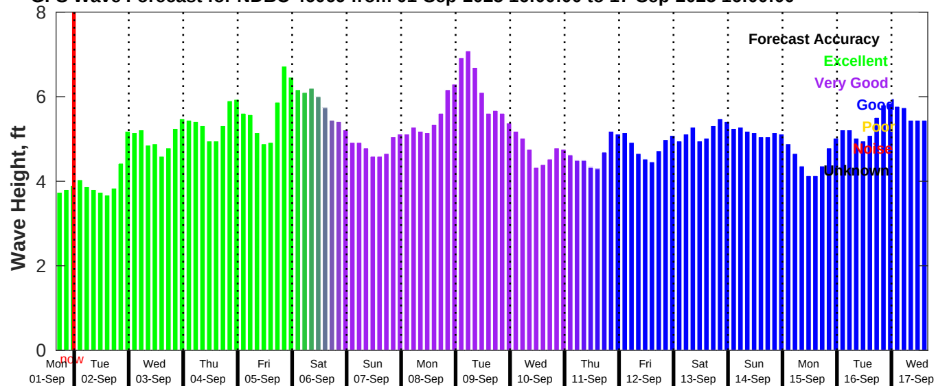
GFS Wave Forecast for NDBC 46069 from 01-Sep-2025 16:00:00 to 17-Sep-2025 16:00:00
