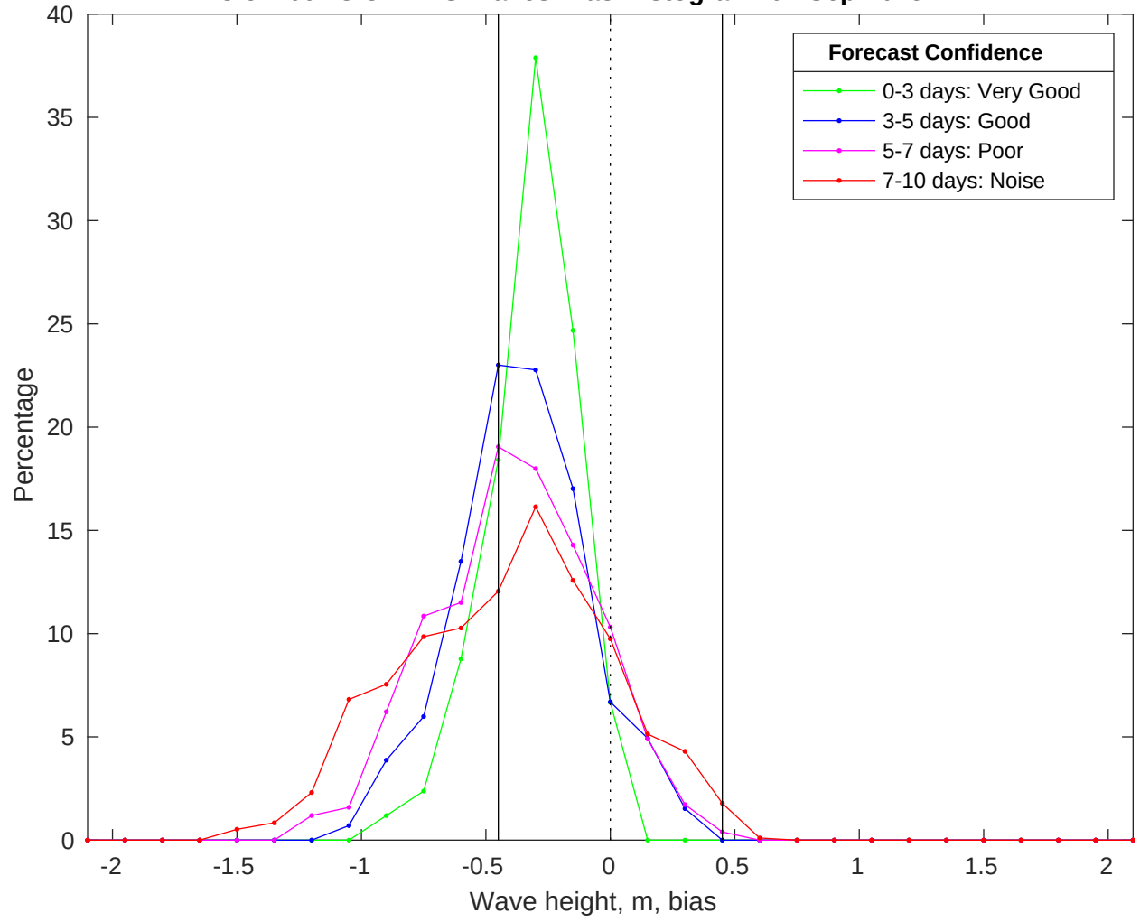
NDBC 51209 vs CMEMS Waves Bias Histogram: 02-Sep-2025
