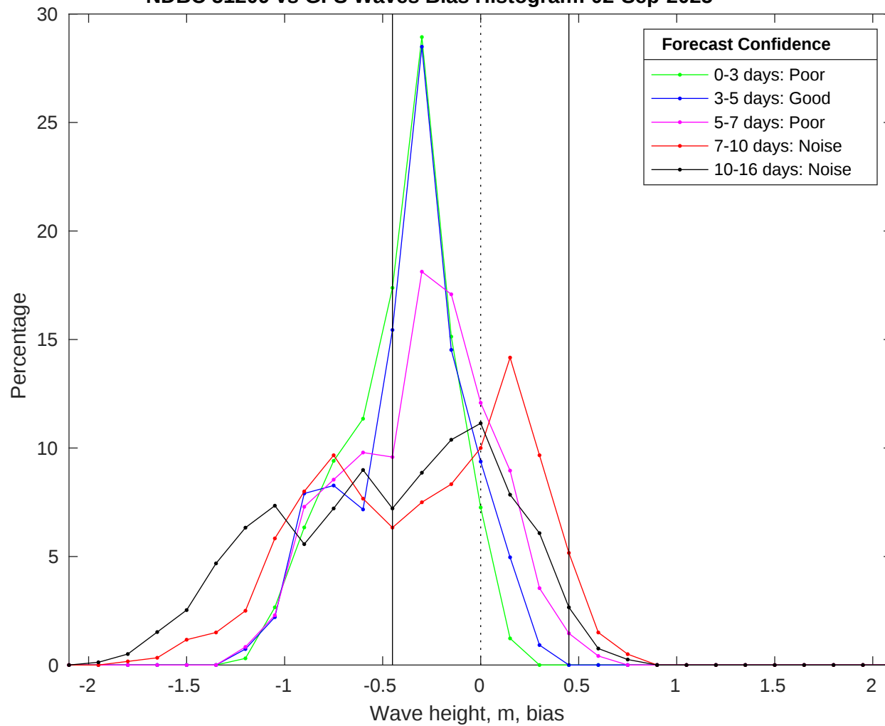
NDBC 51209 vs GFS Waves Bias Histogram: 02-Sep-2025
