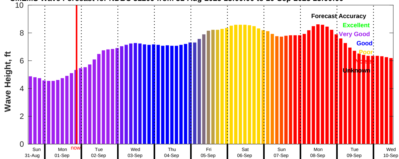
CMEMS Wave Forecast for NDBC 51209 from 31-Aug-2025 13:00:00 to 10-Sep-2025 13:00:00
