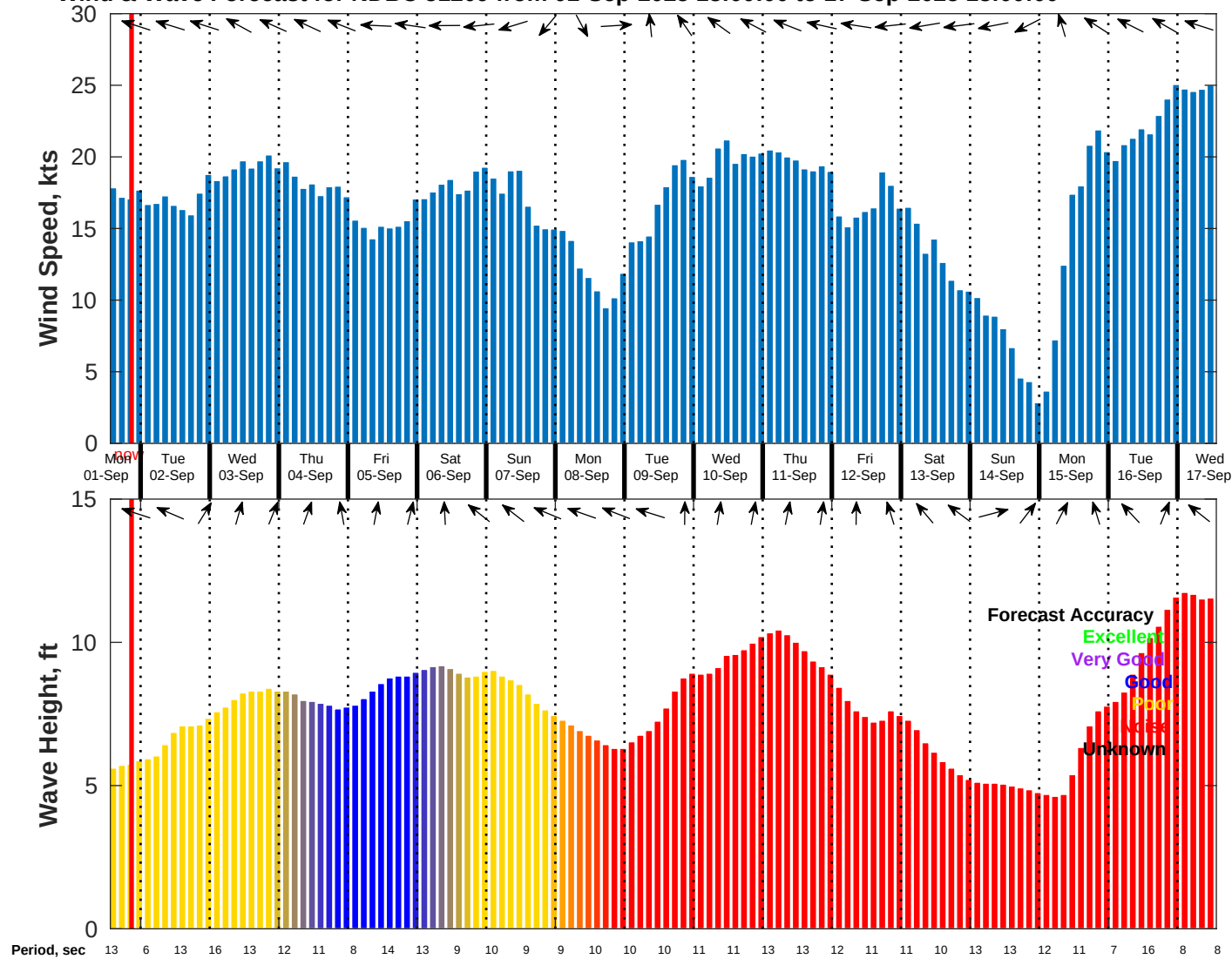
Wind & Wave Forecast for NDBC 51209 from 01-Sep-2025 13:00:00 to 17-Sep-2025 13:00:00
