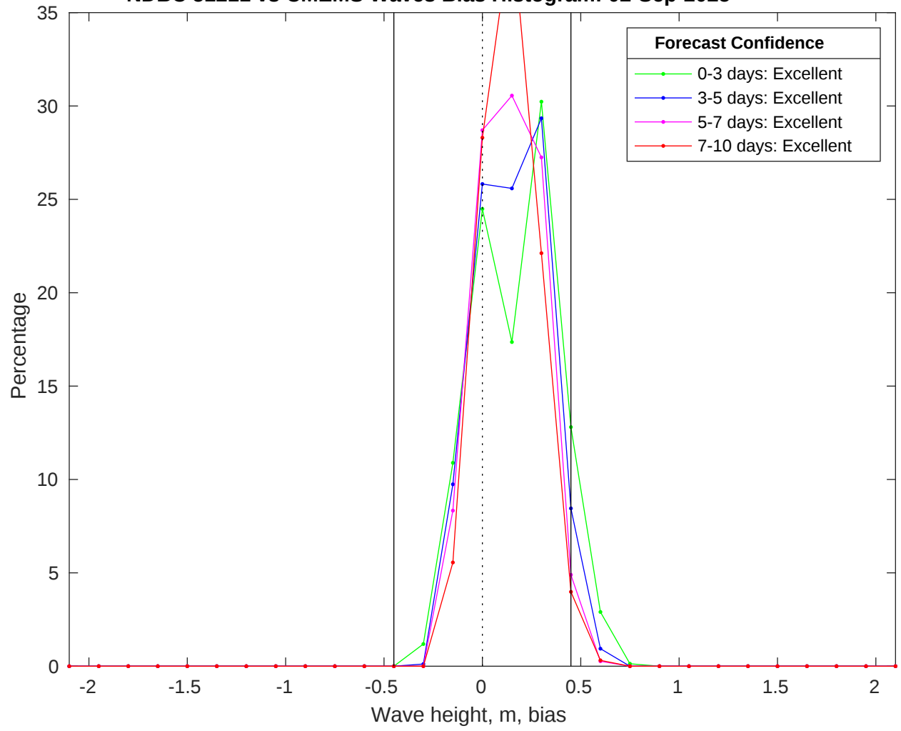
NDBC 51211 vs CMEMS Waves Bias Histogram: 02-Sep-2025
