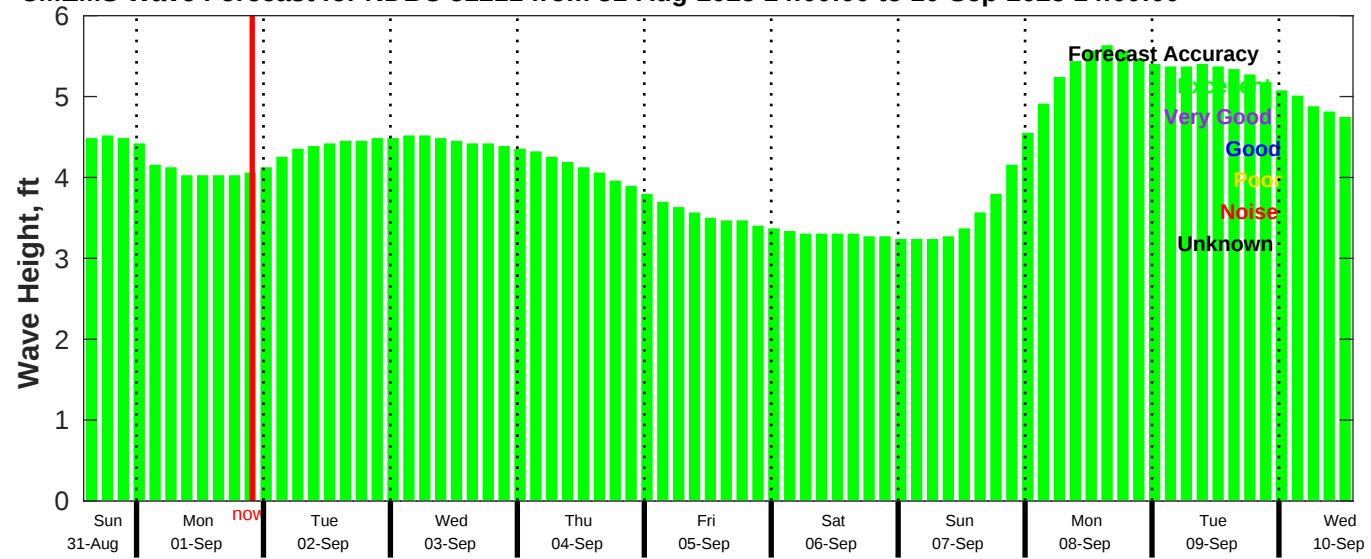
CMEMS Wave Forecast for NDBC 51211 from 31-Aug-2025 14:00:00 to 10-Sep-2025 14:00:00
