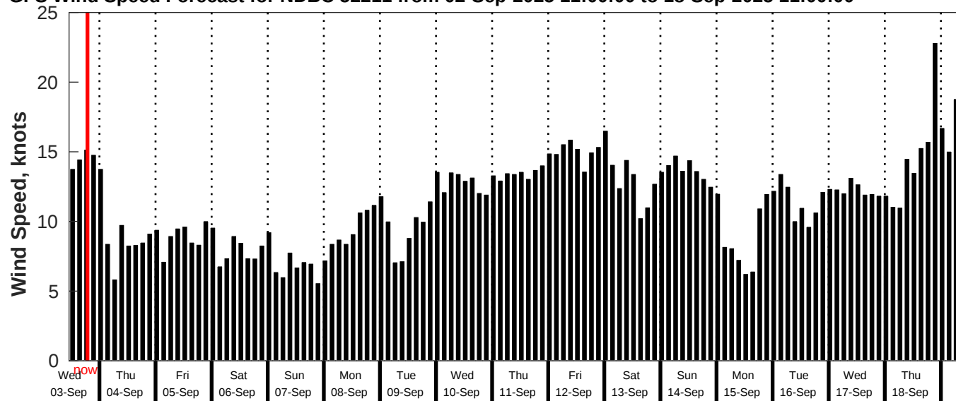
GFS Wind Speed Forecast for NDBC 52211 from 02-Sep-2025 11:00:00 to 18-Sep-2025 11:00:00
