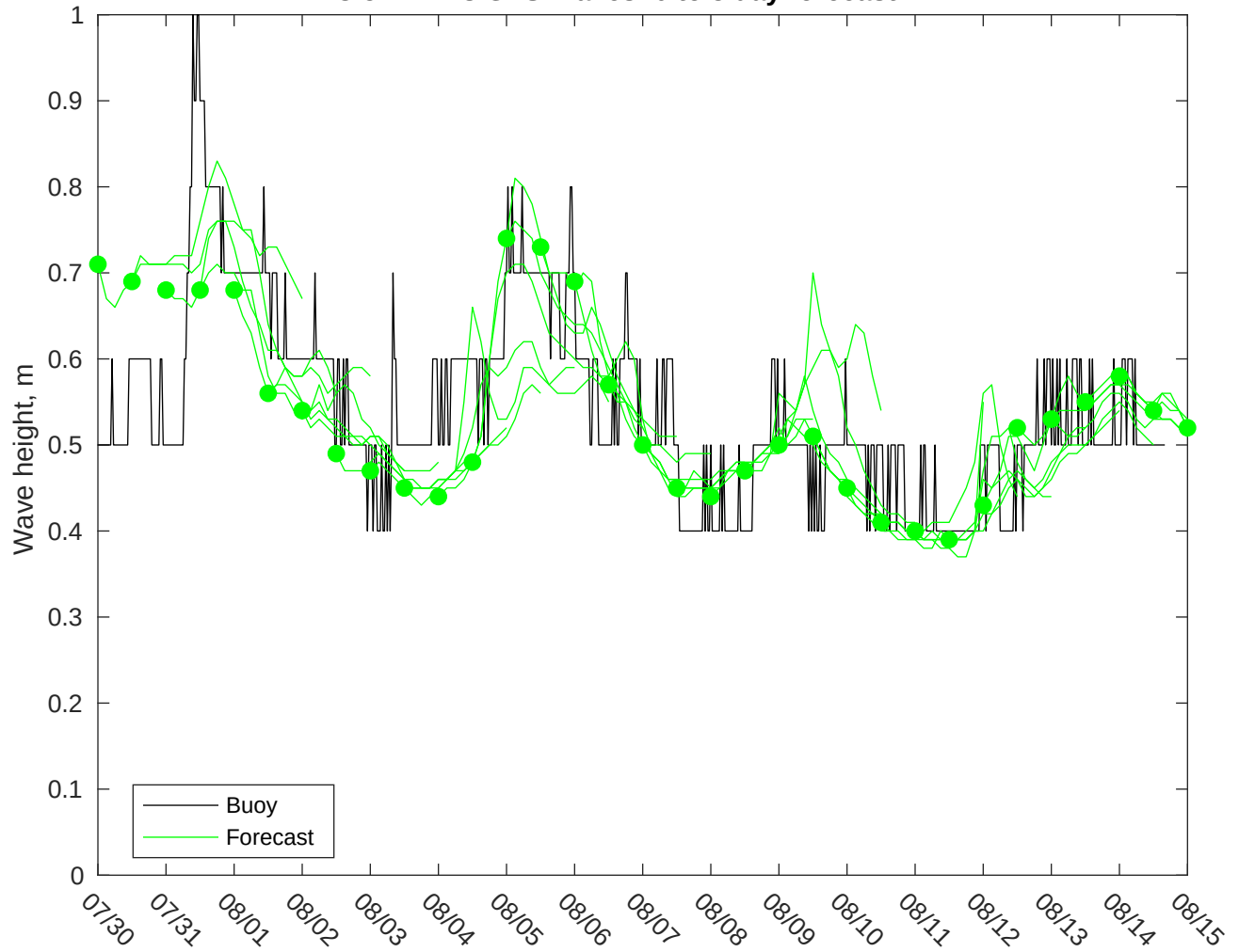
NDBC 52212 vs GFS Waves: 0 to 3 day forecast
