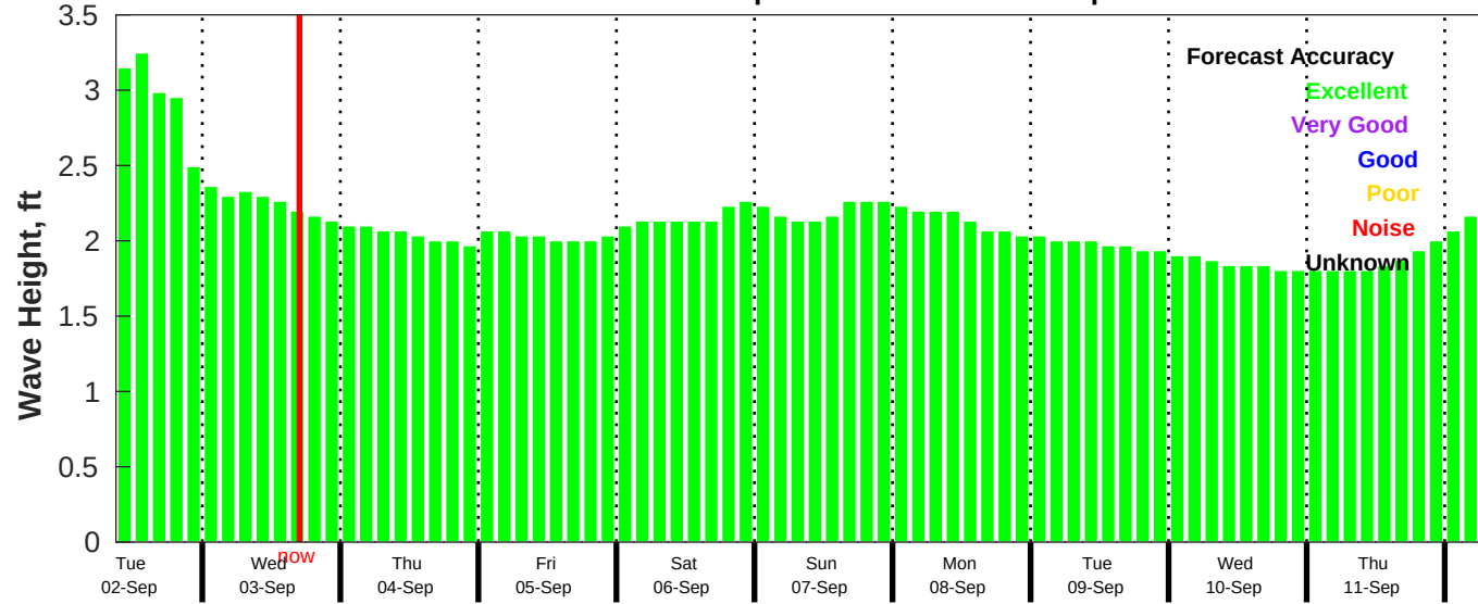
CMEMS Wave Forecast for NDBC 52212 from 01-Sep-2025 09:00:00 to 11-Sep-2025 09:00:00
