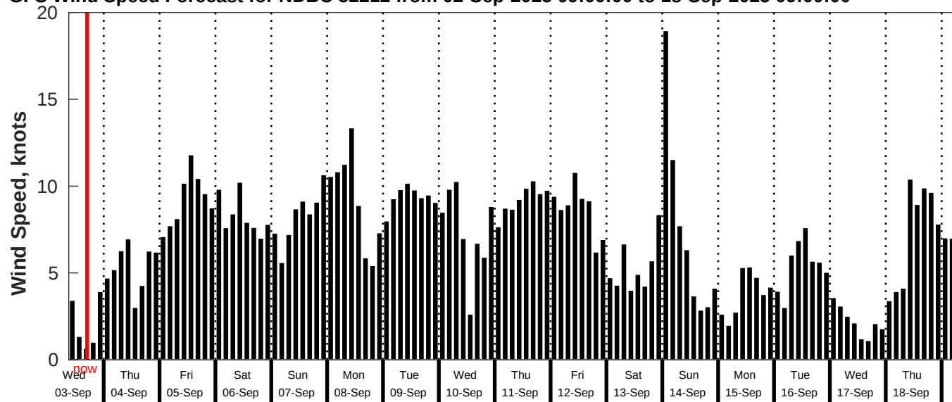
GFS Wind Speed Forecast for NDBC 52212 from 02-Sep-2025 09:00:00 to 18-Sep-2025 09:00:00
