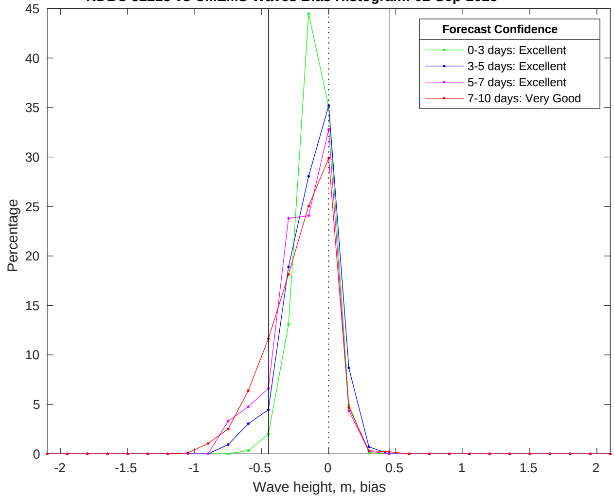
NDBC 52213 vs CMEMS Waves Bias Histogram: 02-Sep-2025
