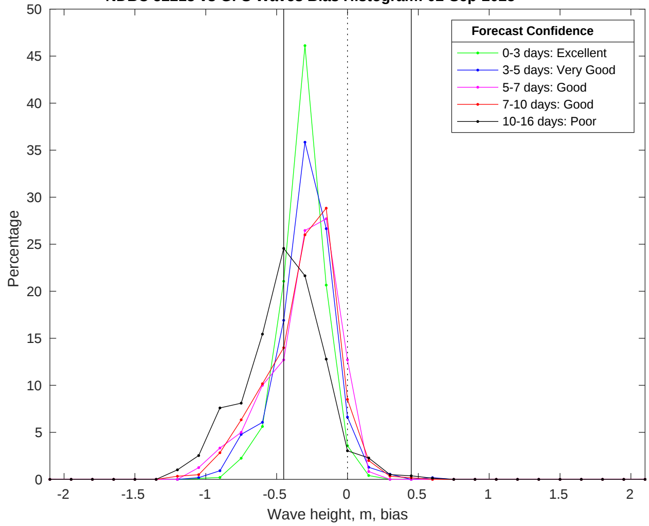
NDBC 52213 vs GFS Waves Bias Histogram: 02-Sep-2025
