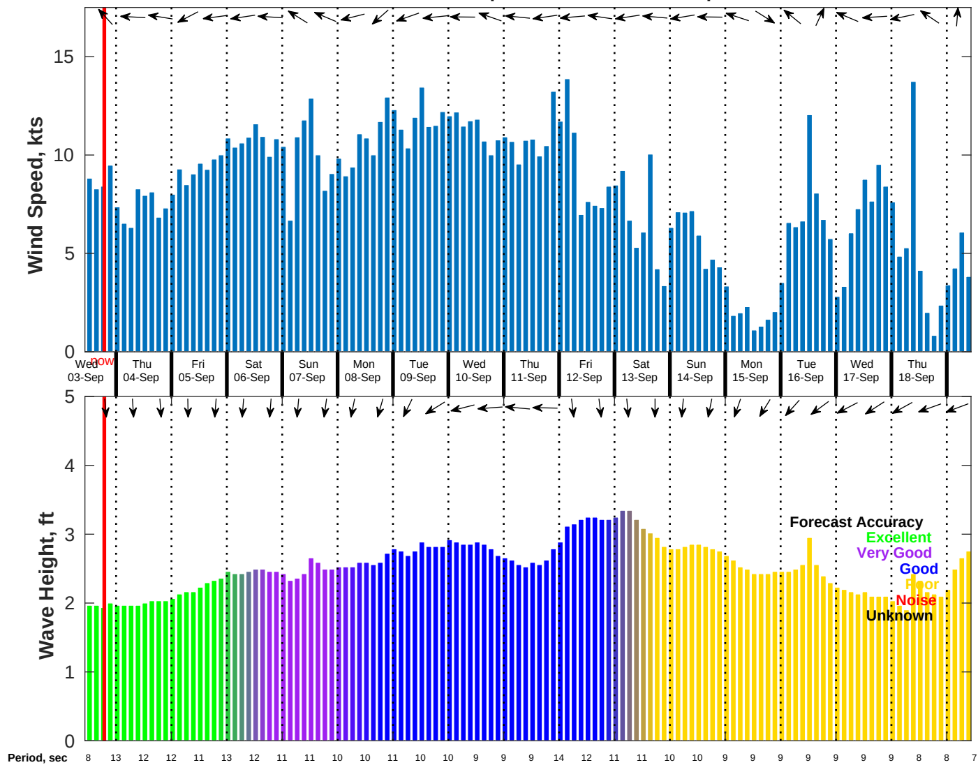
Wind & Wave Forecast for NDBC 52213 from 02-Sep-2025 11:00:00 to 18-Sep-2025 11:00:00
