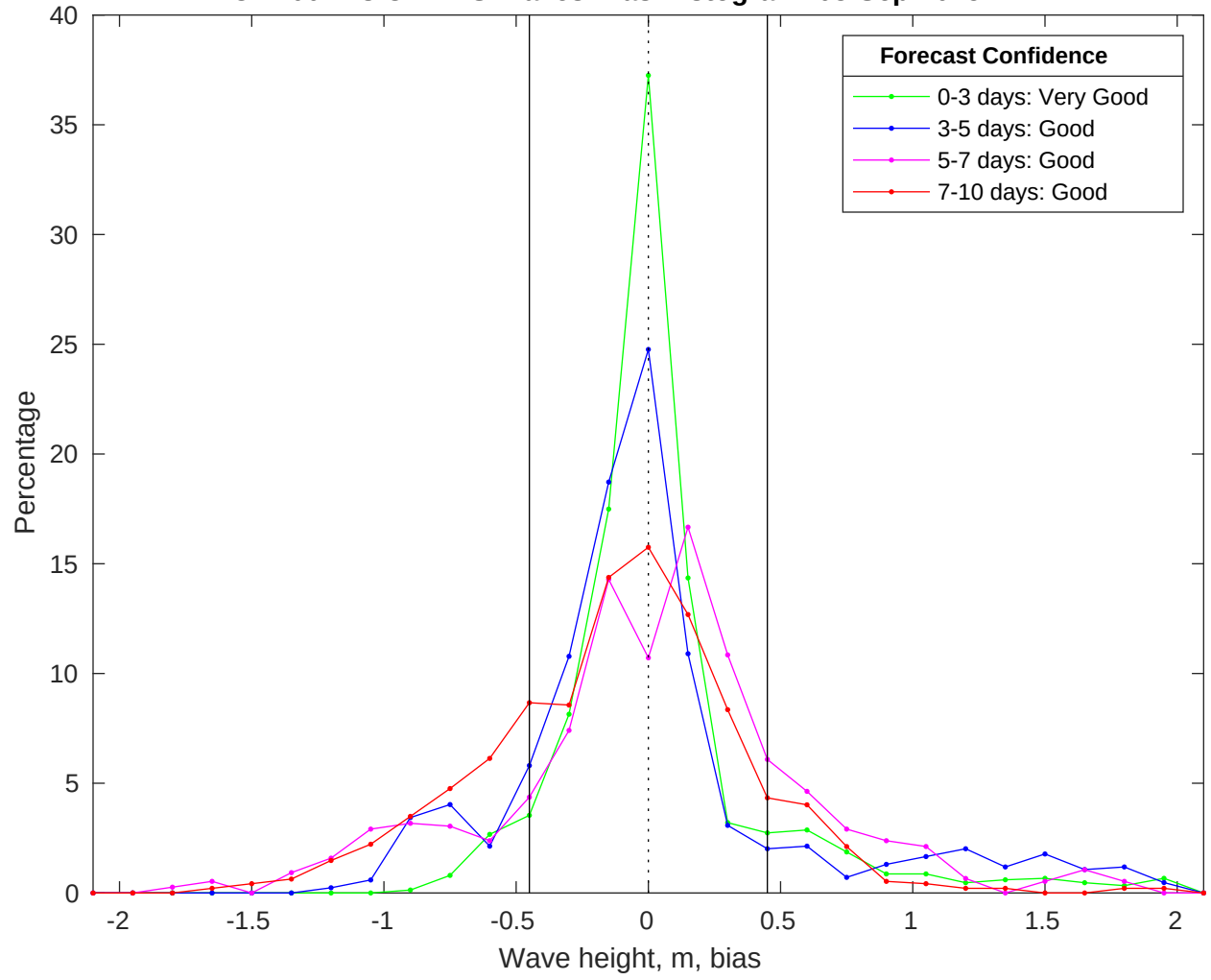
NDBC 41004 vs CMEMS Waves Bias Histogram: 03-Sep-2025
