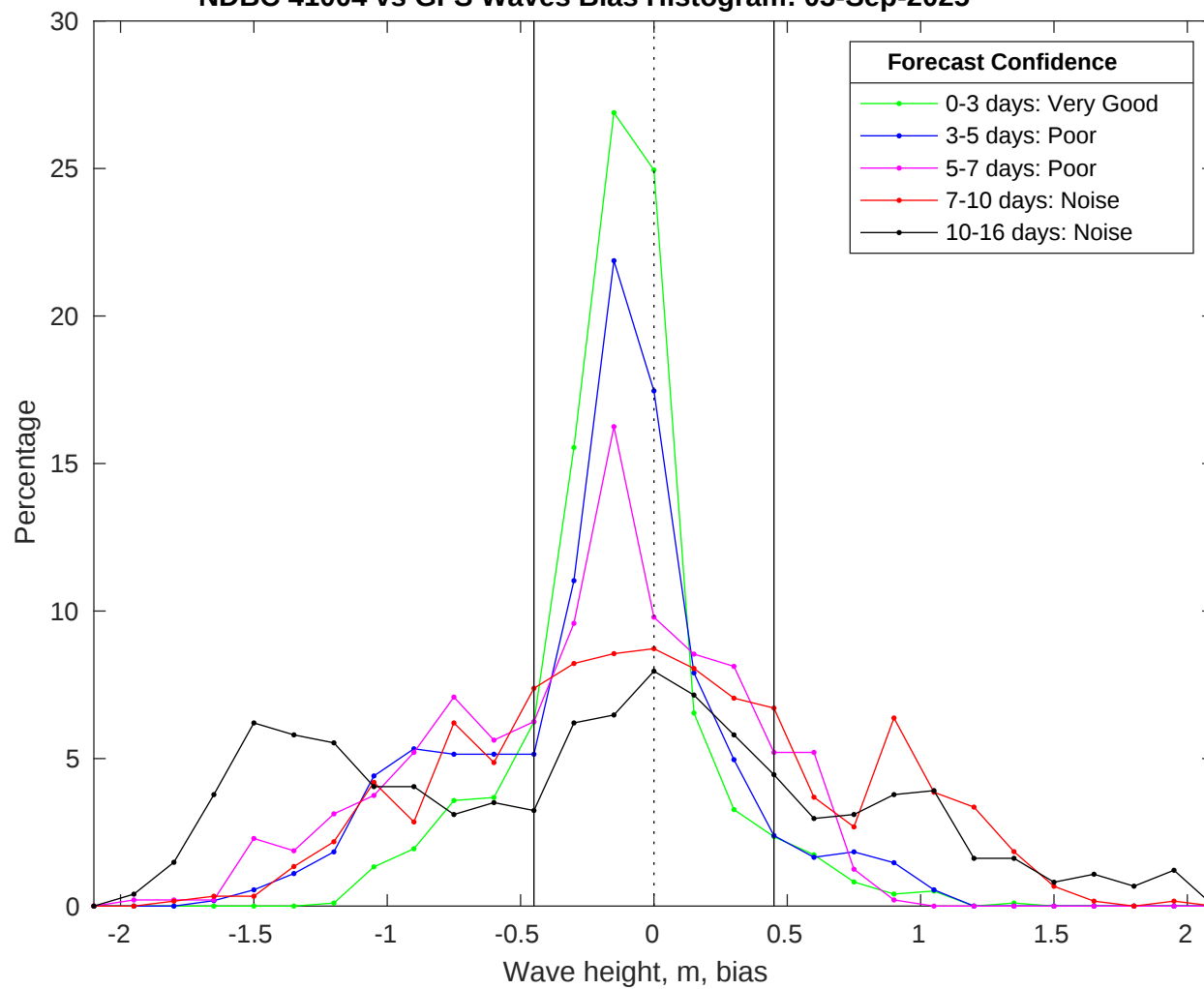
NDBC 41004 vs GFS Waves Bias Histogram: 03-Sep-2025
