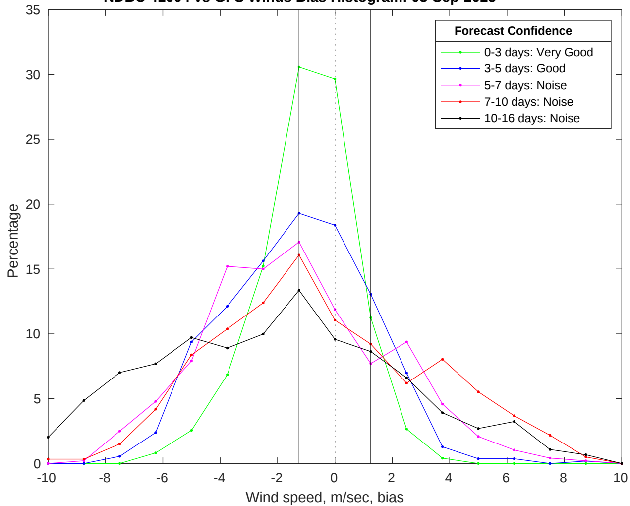
NDBC 41004 vs GFS Winds Bias Histogram: 03-Sep-2025
