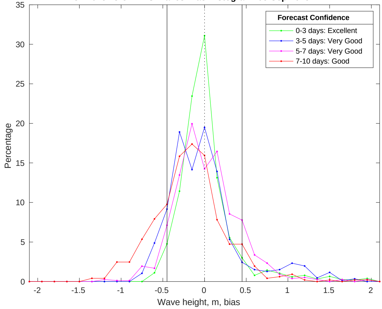
NDBC 41013 vs CMEMS Waves Bias Histogram: 03-Sep-2025
