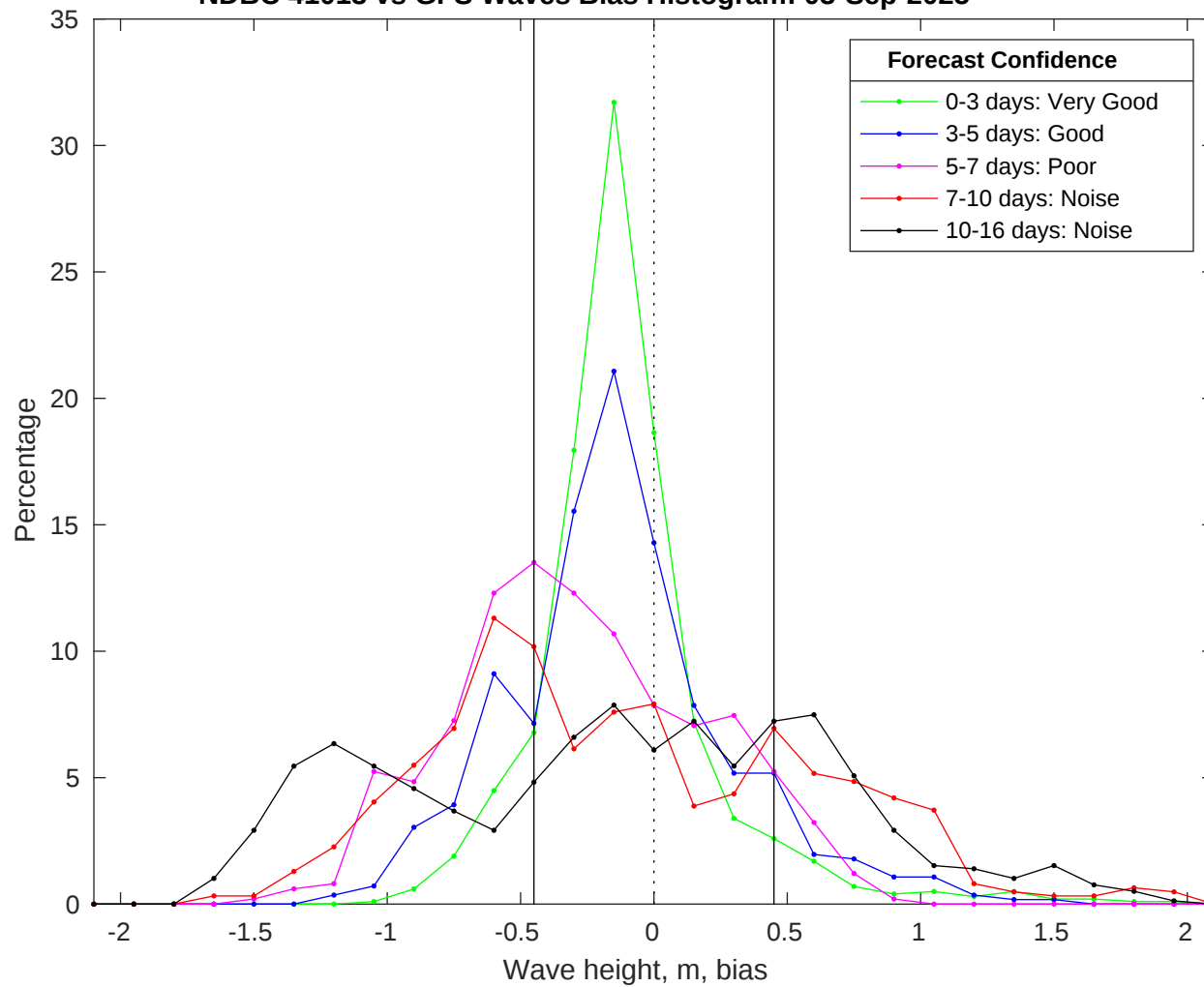
NDBC 41013 vs GFS Waves Bias Histogram: 03-Sep-2025
