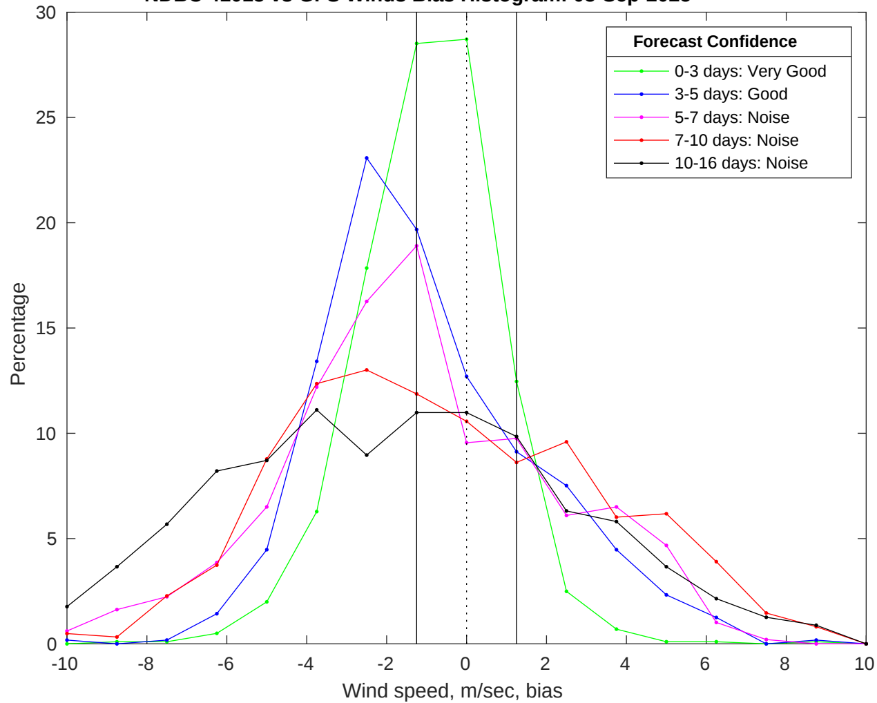
NDBC 41013 vs GFS Winds Bias Histogram: 03-Sep-2025
