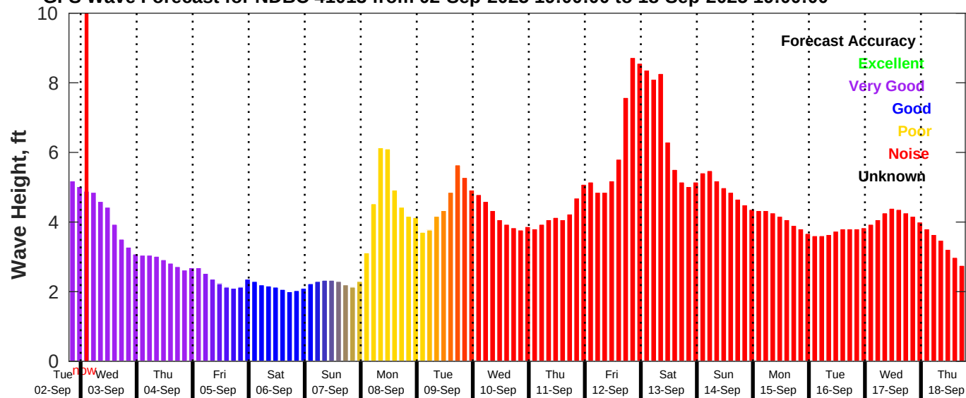
GFS Wave Forecast for NDBC 41013 from 02-Sep-2025 19:00:00 to 18-Sep-2025 19:00:00
