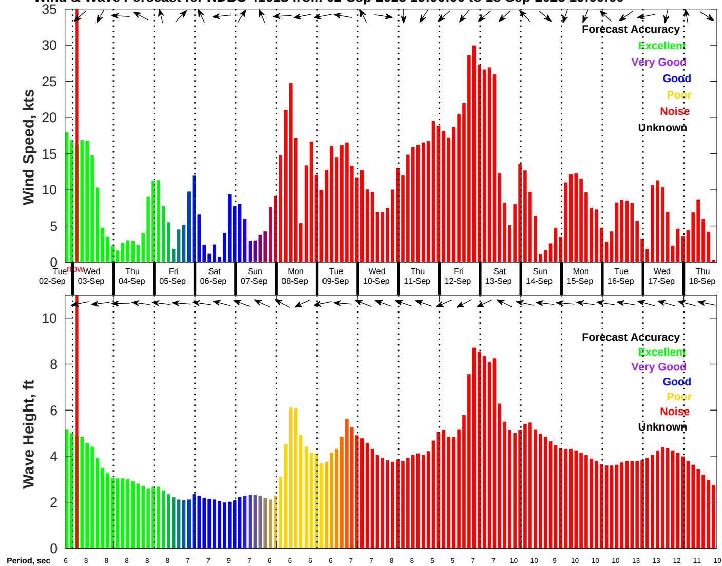
Wind & Wave Forecast for NDBC 41013 from 02-Sep-2025 19:00:00 to 18-Sep-2025 19:00:00
