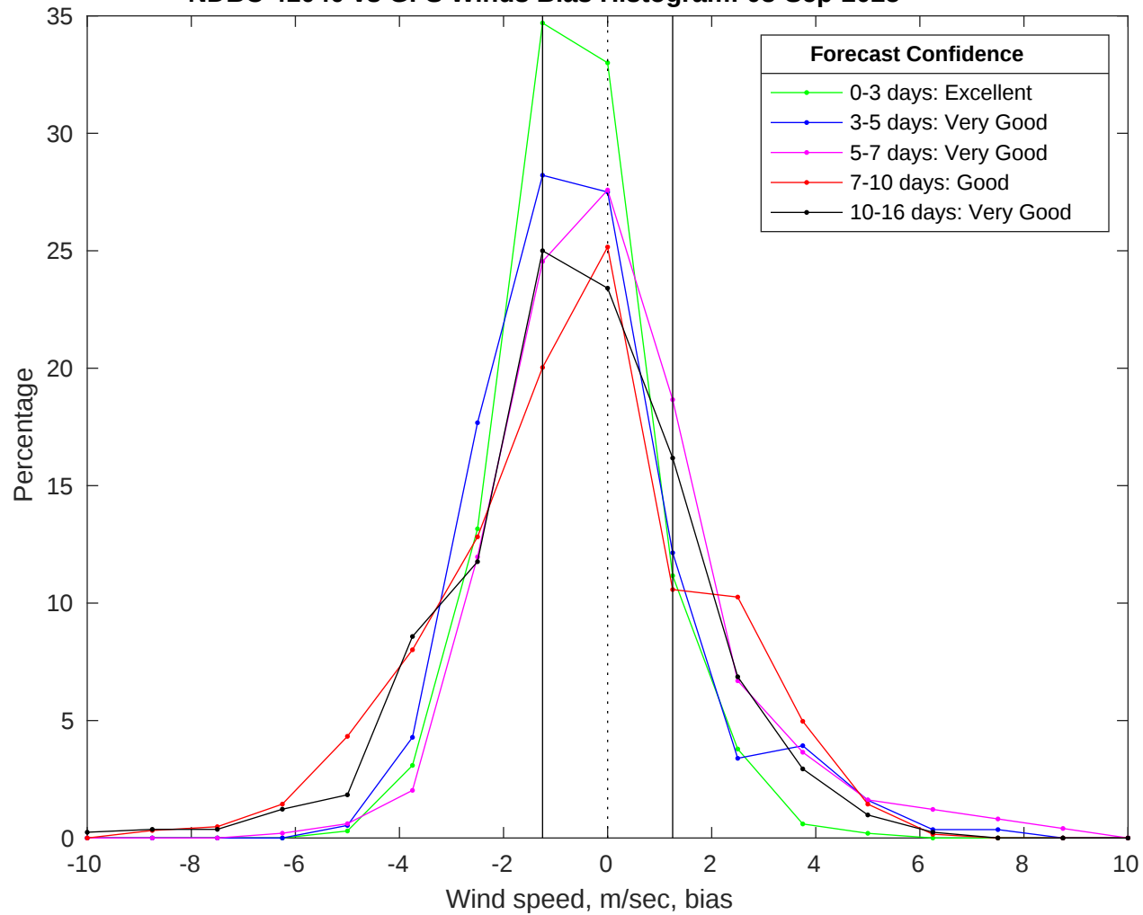
NDBC 41040 vs GFS Winds Bias Histogram: 03-Sep-2025
