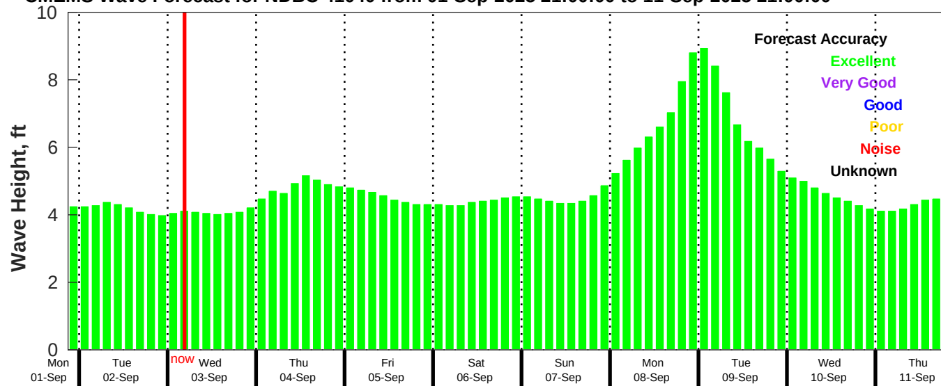
CMEMS Wave Forecast for NDBC 41040 from 01-Sep-2025 21:00:00 to 11-Sep-2025 21:00:00
