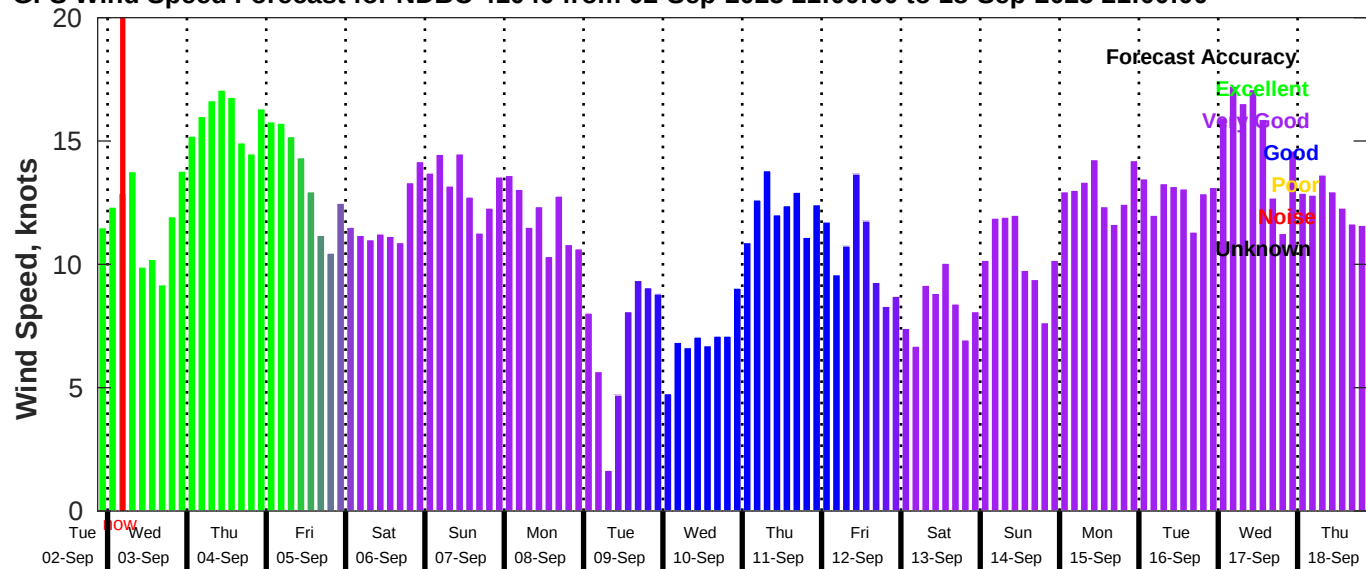
GFS Wind Speed Forecast for NDBC 41040 from 02-Sep-2025 21:00:00 to 18-Sep-2025 21:00:00
