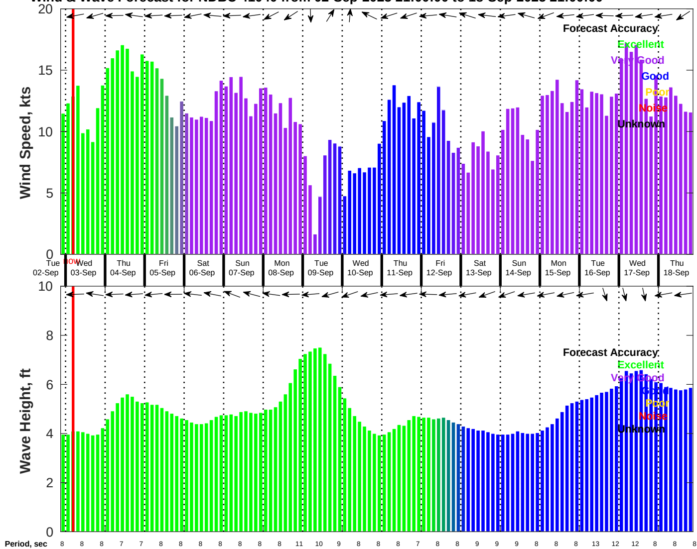
Wind & Wave Forecast for NDBC 41040 from 02-Sep-2025 21:00:00 to 18-Sep-2025 21:00:00
