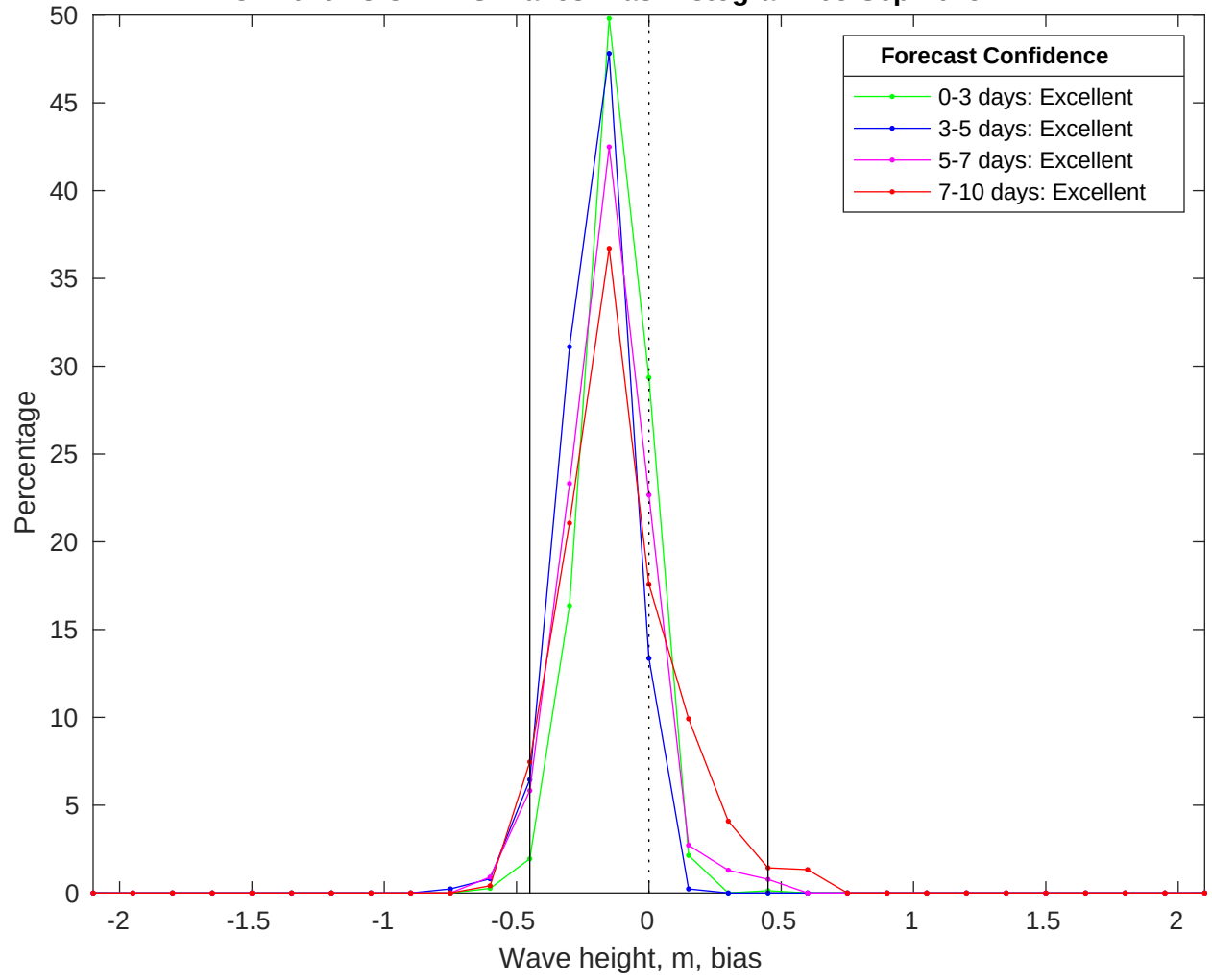
NDBC 42019 vs CMEMS Waves Bias Histogram: 03-Sep-2025
