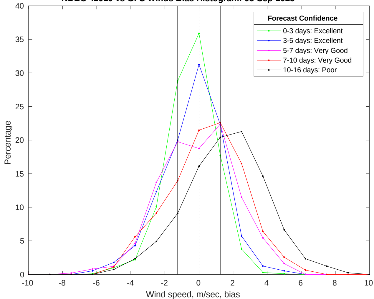
NDBC 42019 vs GFS Winds Bias Histogram: 03-Sep-2025
