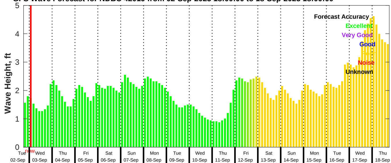
GFS Wave Forecast for NDBC 42019 from 02-Sep-2025 18:00:00 to 18-Sep-2025 18:00:00
