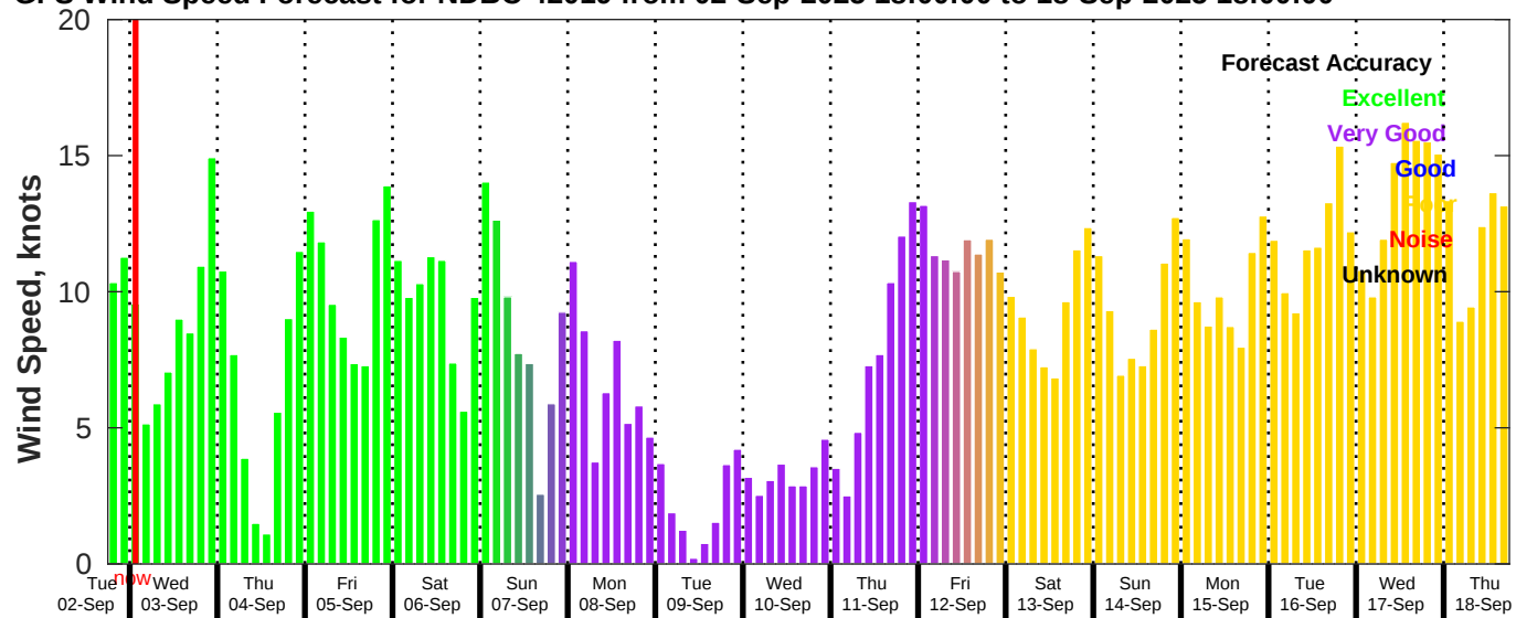
GFS Wind Speed Forecast for NDBC 42019 from 02-Sep-2025 18:00:00 to 18-Sep-2025 18:00:00
