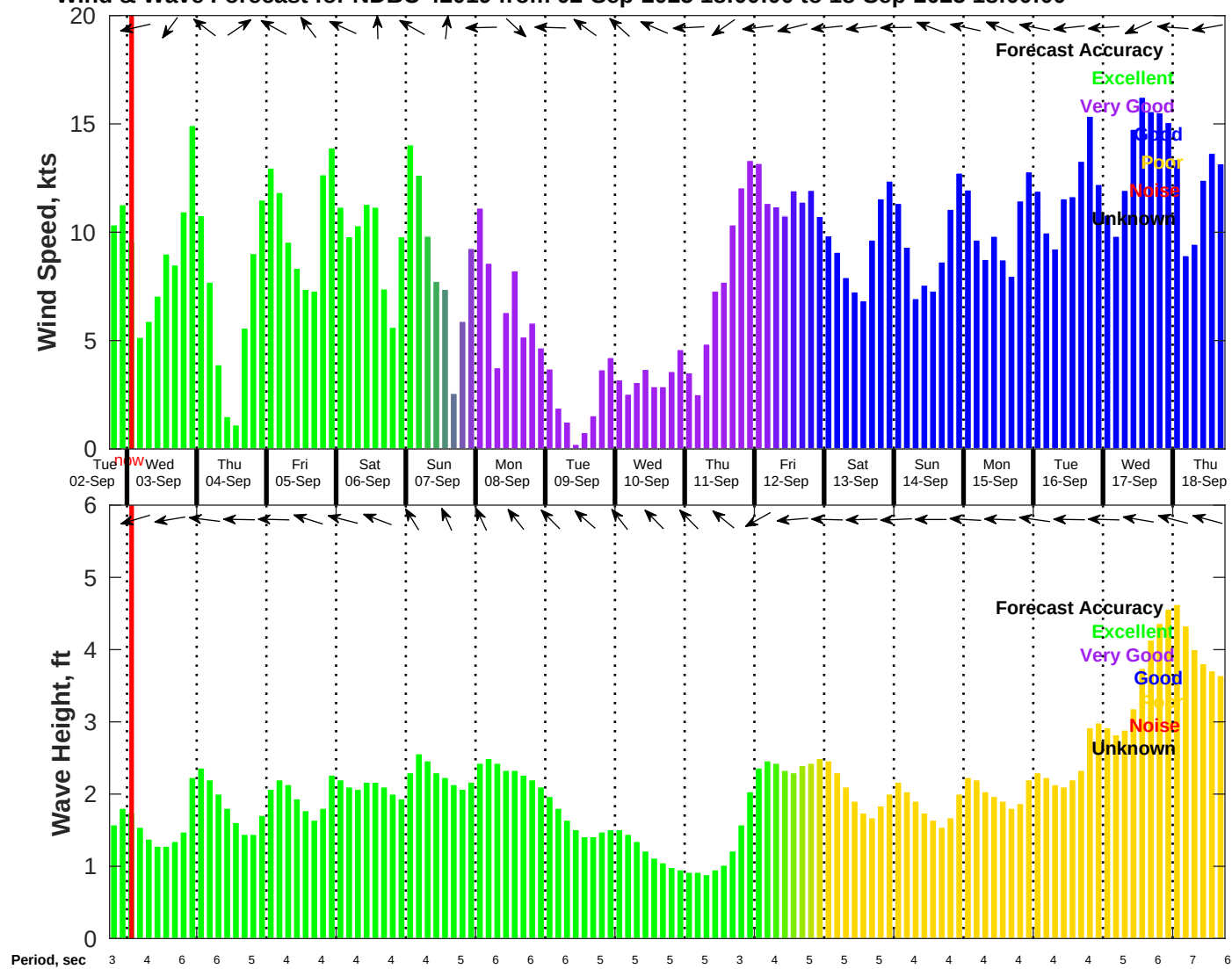
Wind & Wave Forecast for NDBC 42019 from 02-Sep-2025 18:00:00 to 18-Sep-2025 18:00:00
