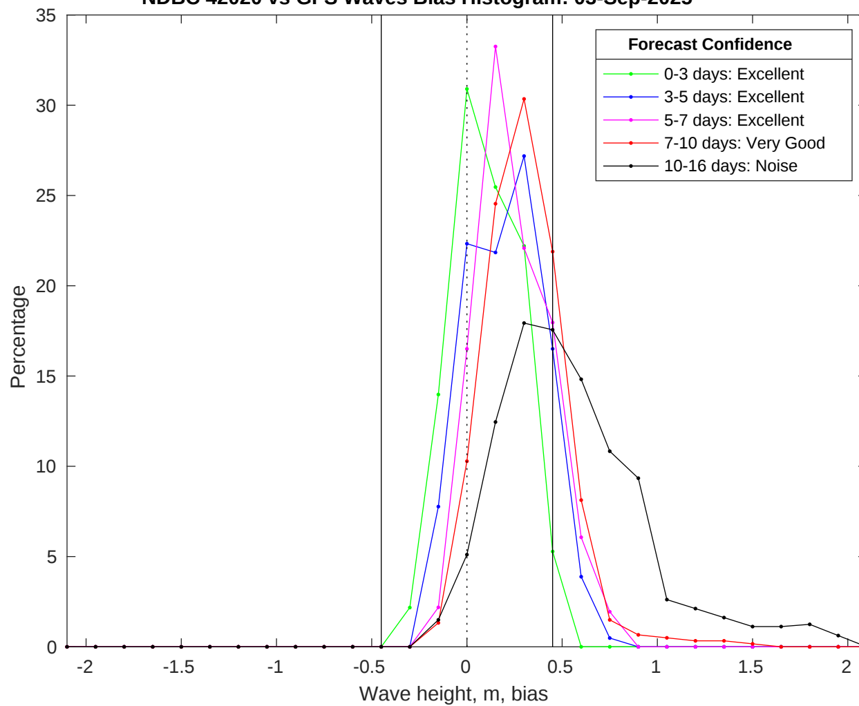
NDBC 42020 vs GFS Waves Bias Histogram: 03-Sep-2025
