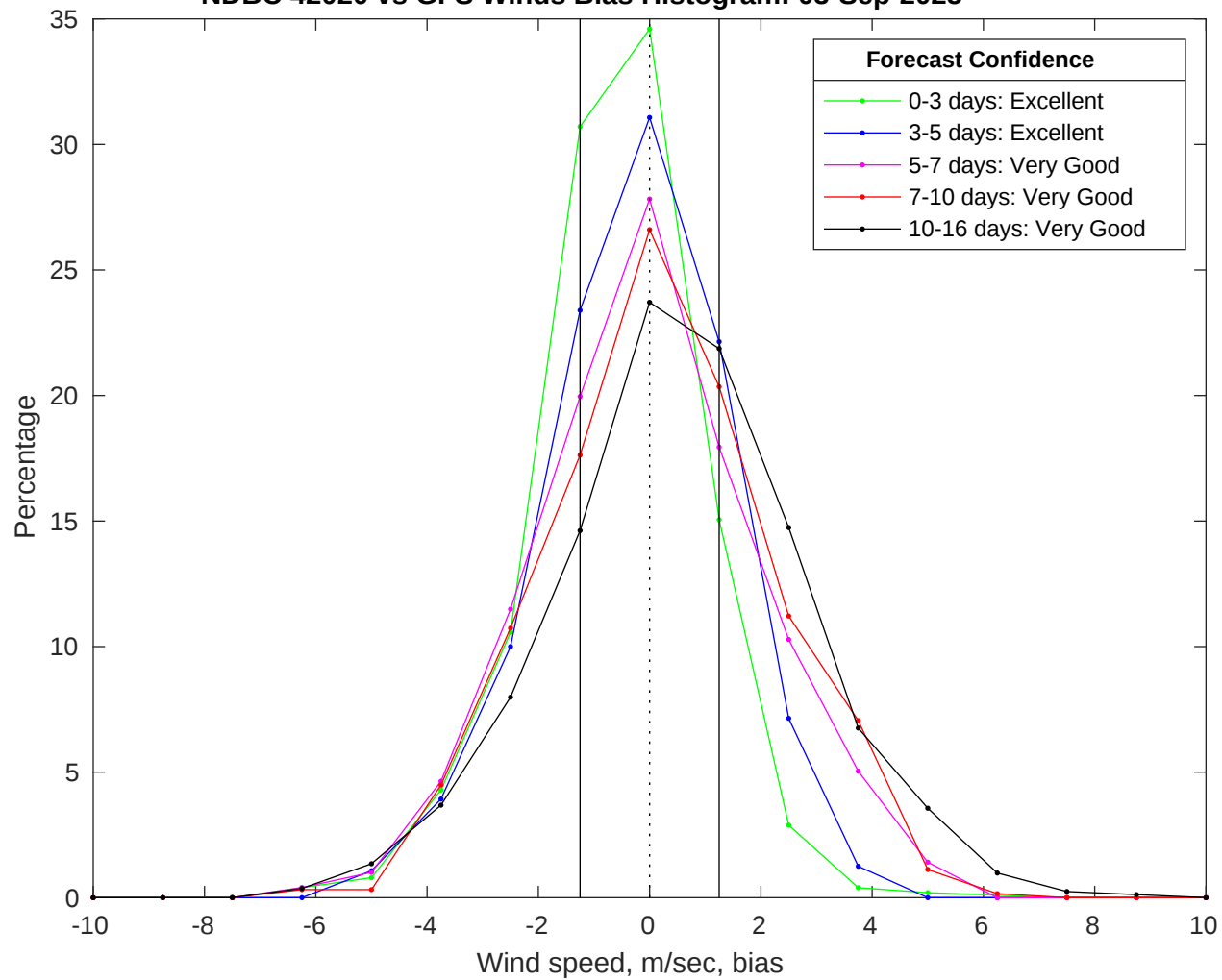
NDBC 42020 vs GFS Winds Bias Histogram: 03-Sep-2025
