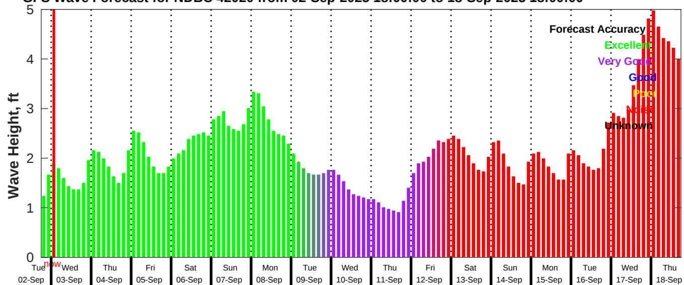
GFS Wave Forecast for NDBC 42020 from 02-Sep-2025 18:00:00 to 18-Sep-2025 18:00:00
