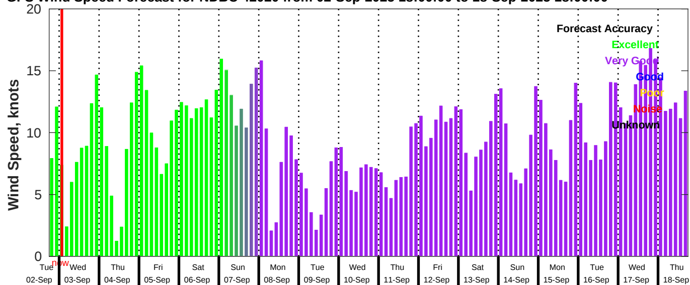
GFS Wind Speed Forecast for NDBC 42020 from 02-Sep-2025 18:00:00 to 18-Sep-2025 18:00:00
