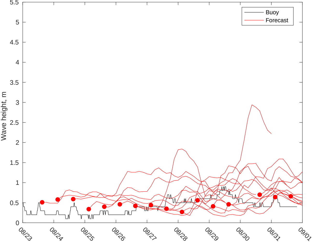
NDBC 42035 vs GFS Waves: 10 to 16 day forecast
